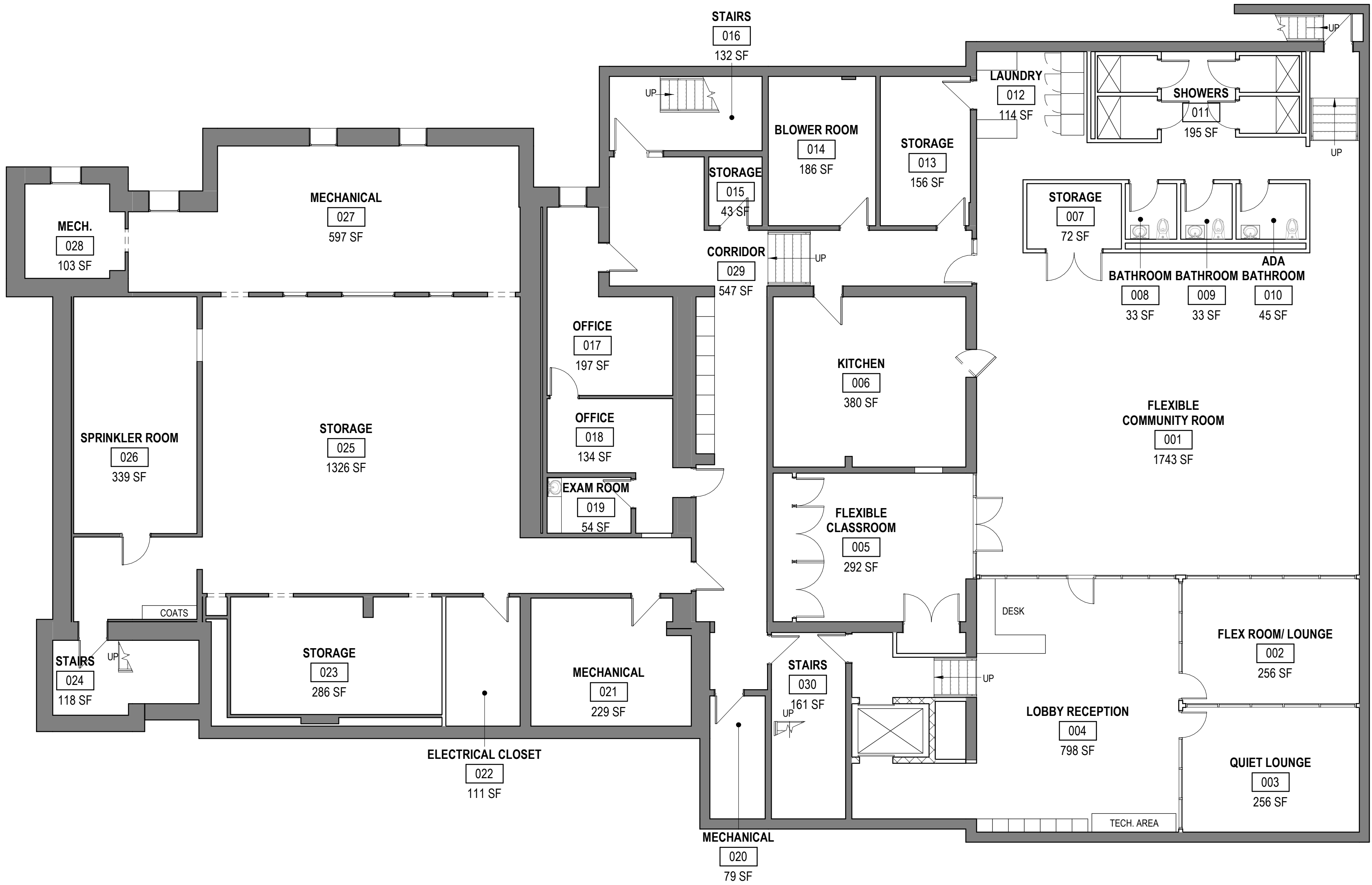
1 architectural plan - basement 1/8" = 1'-0"
